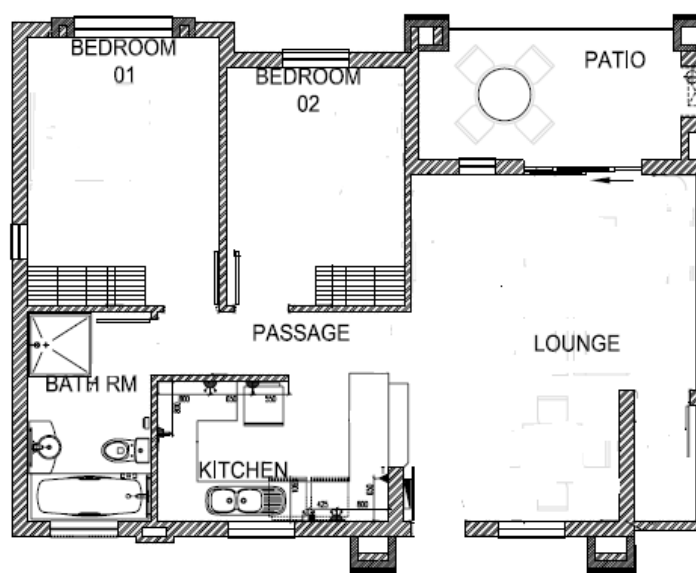
2 Bedroom Ground Floor
