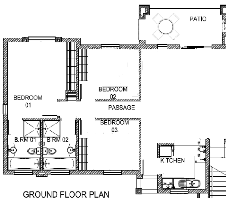
3 Bedroom Ground Floor
